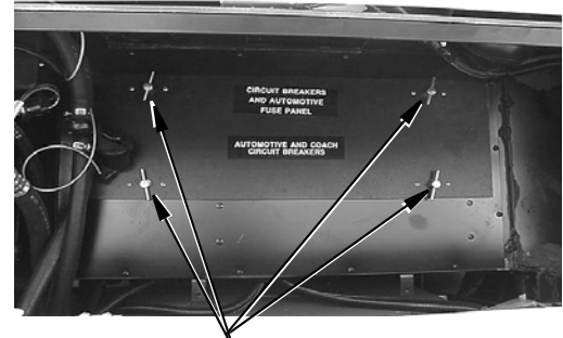
Twist Locks to Remove Cover
