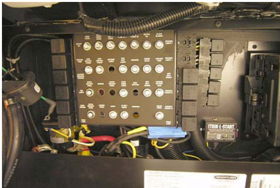
Chassis Fuses/Breakers & Relays (Behind "Hood" Panel)
