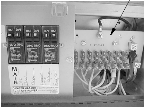
12-Volt House Fuses
