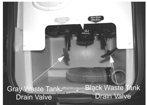
Holding Tank Drain Valves (Located in holding tank compartment) -Typical View
