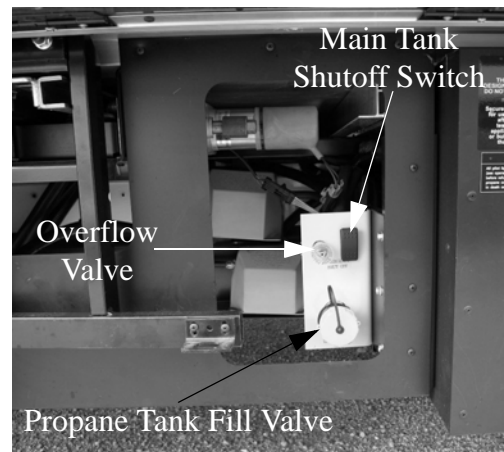
Propane Gas Access (Located in driver side compartment) -Typical View
