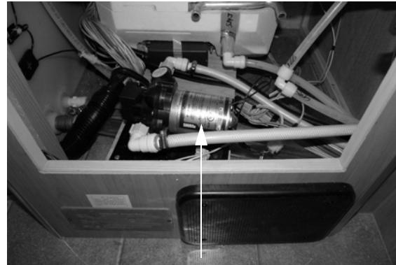
Water Pump (Located behind removable access panel below wardrobe) -Model 24J shown
