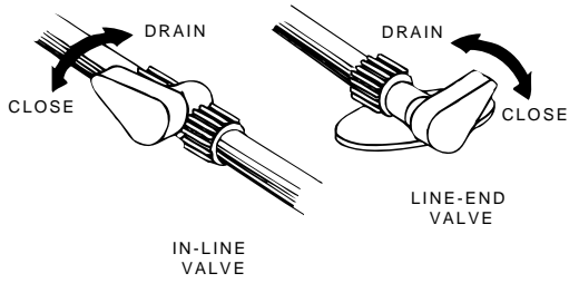
Waterline Drain Valves (Typical)
