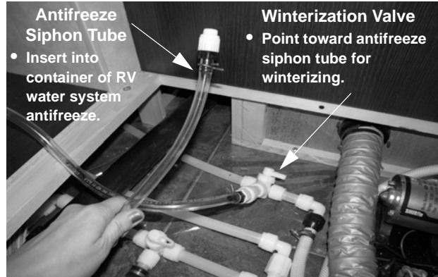
Antifreeze Siphon Tube and Winterization Valve
