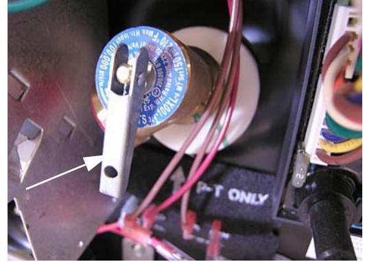
•Lift handle straight out to open P-T valve when water heater is cold -Typical View
