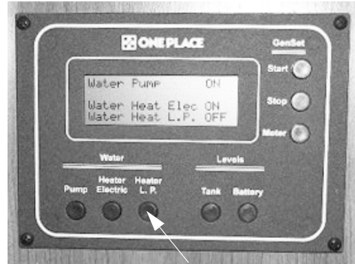
Propane Gas Water Heater Switch (Located on OnePlace® monitor panel)
