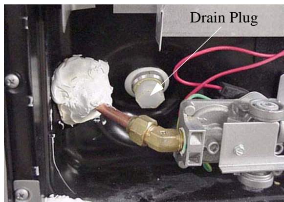
Water Heater Service Access -Typical View
