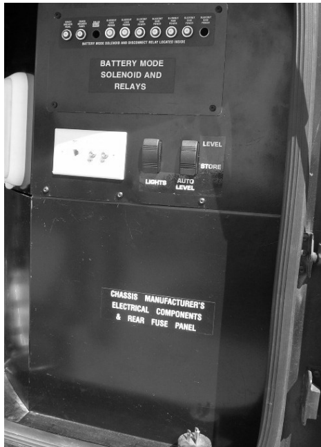
Rear Chassis Control Module - CCM (Remove panel to access)
