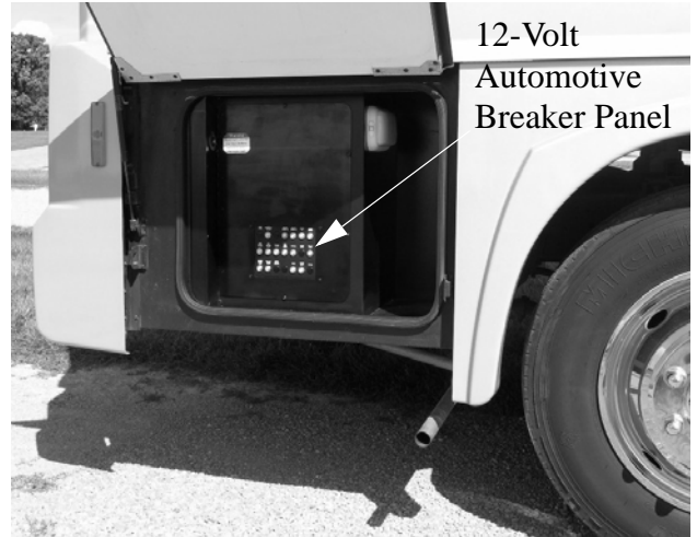
12-Volt Automotive Breaker Panel Front Chassis Control Module - CCM (Remove panel to access)
