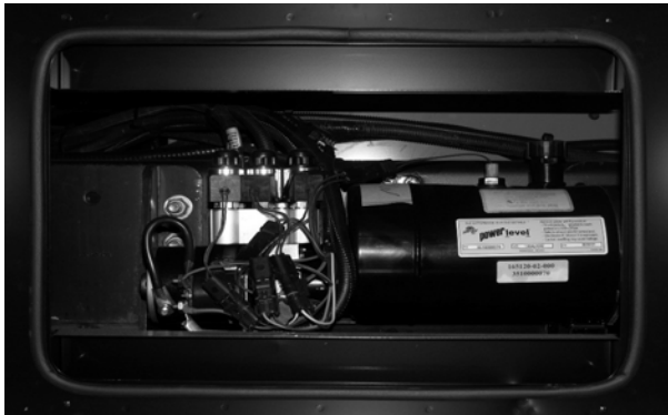
Hydraulic Pump (Behind right front compartment access panel) - Typical View
